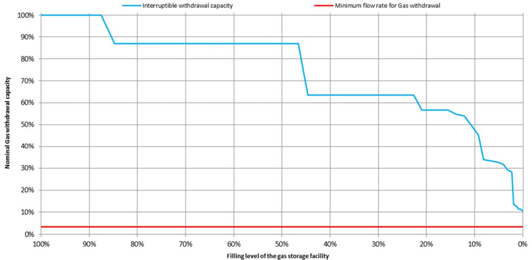
Gas withdrawal curve for GSF Kawerna – Interruptible Storage Services
